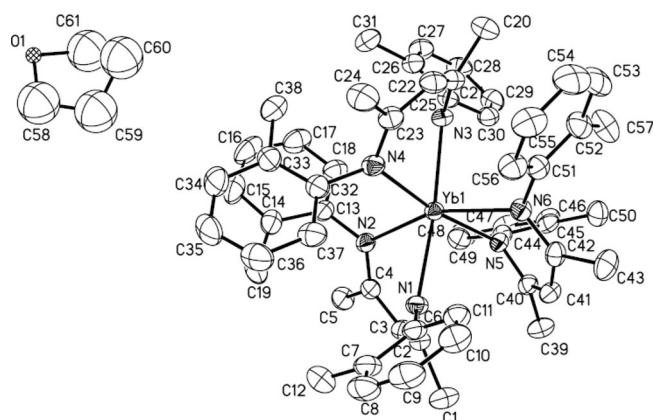
Figure 3. ORTEP diagram of 3 showing atom-numbering scheme; thermal ellipsoids are drawn at the 10% probability level. Hydrogen atoms are omitted for clarity.
