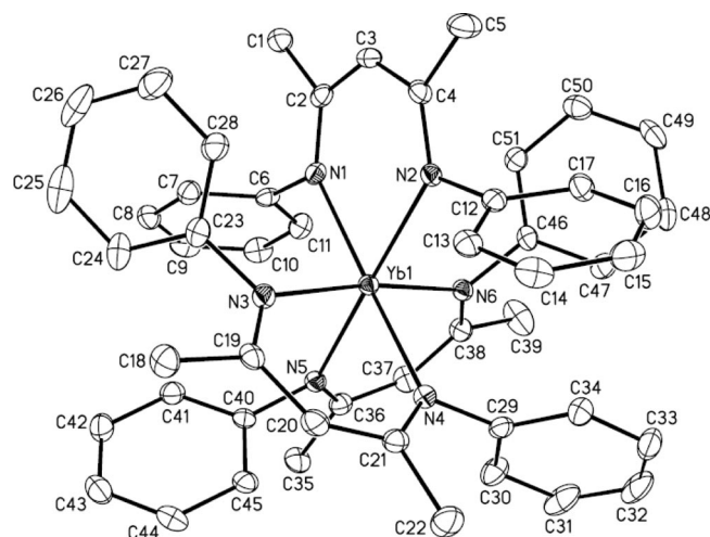
Figure 1. ORTEP diagram of 1 showing atom-numbering scheme; thermal ellipsoids are drawn at the 10% probability level. Hydrogen atoms are omitted for clarity.
