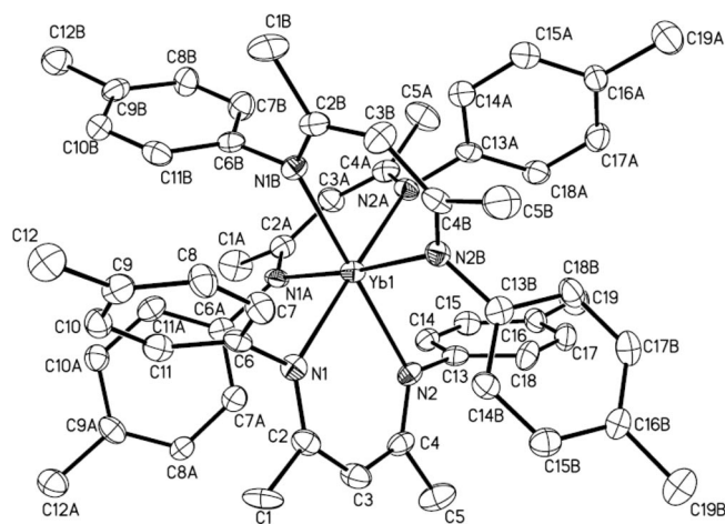
Figure 2. ORTEP diagram of 2 showing atom-numbering scheme; thermal ellipsoids are drawn at the 10% probability level. Hydrogen atoms are omitted for clarity.
